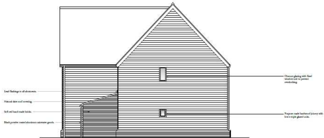
SIDE ELEVATION (WEST FACING)
